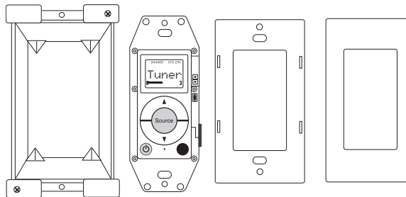
Electrical Box KPL Keypad Back Plate Trim Plate
