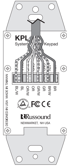
CAT-5 to KPL Connection
